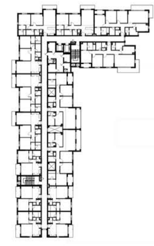
LEVEL 04,05,06,07,08
