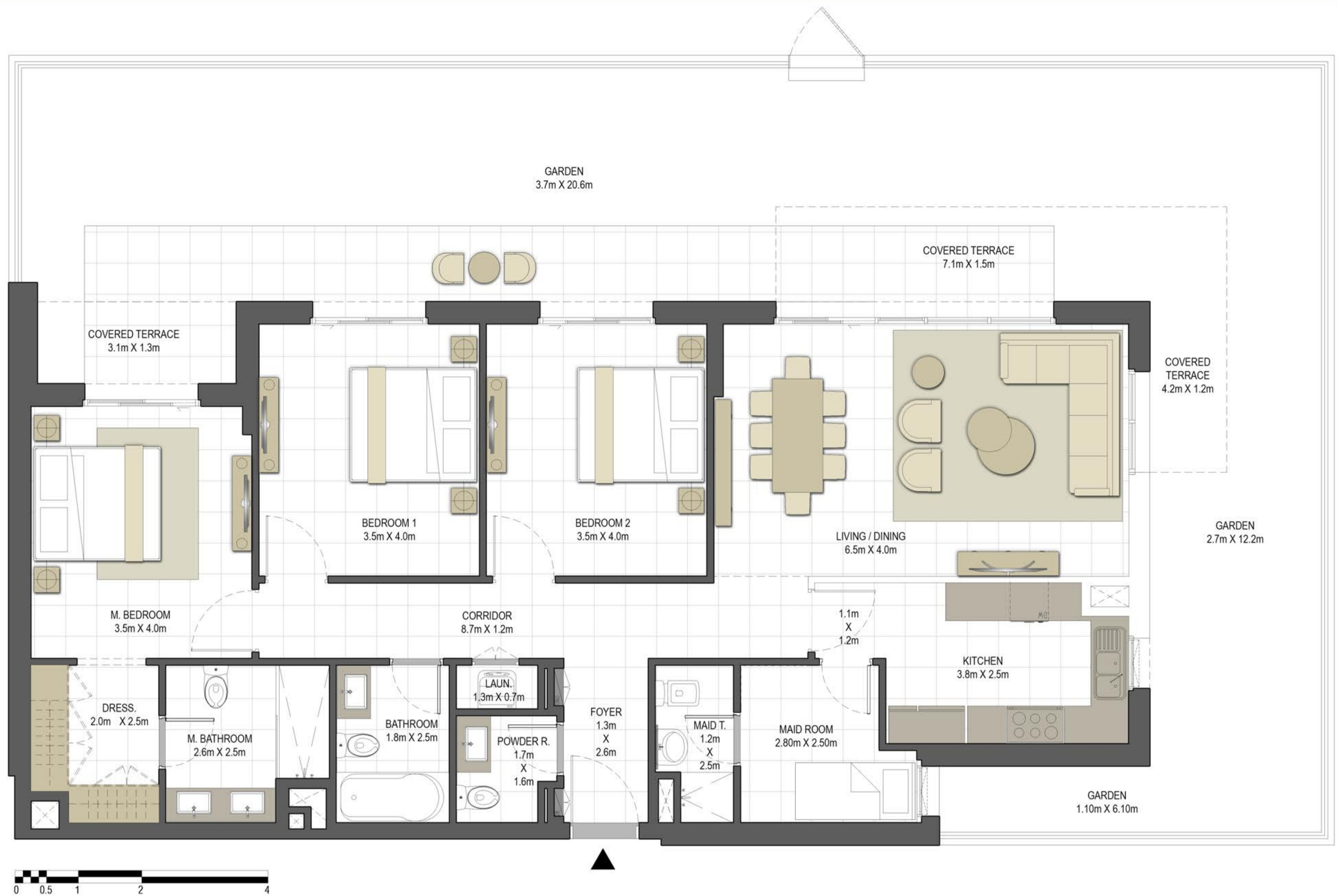
LEVEL G
