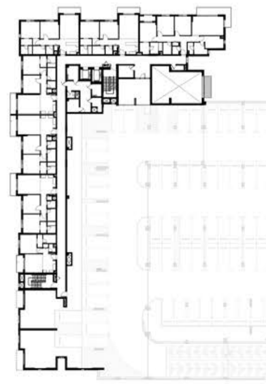
LEVEL 01
